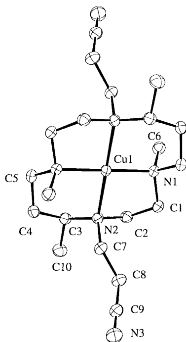
Fig. 4 An ORTEP drawing of the molecular structure of [CuL 8 ][ClO 4 ] 2 6 along with the atom numbering scheme.
