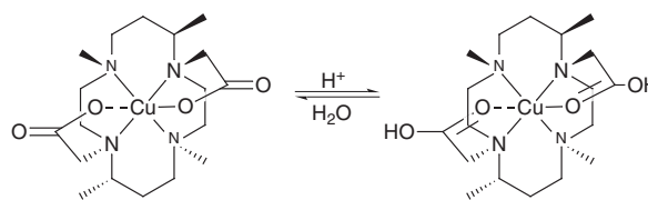
Scheme 1 Structural rearrangement of [\text{Cu}(\text{H}_2\text{L}^9)](\text{ClO}_4)_2 in aqueous solution.
