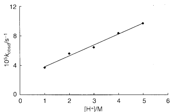
Fig. 8 Plot of k_{\text{obs}} vs. [\text{H}^+] for the dissociation of complex 6 at 25.0 \pm 0.1^\circ\text{C} and I = 5.0 \text{ mol dm}^{-3} ( \text{NaCl} + \text{HCl} ). The circles are the experimental results; the line is calculated from k_{\text{obs}} = k_{23}K_{12}[\text{H}^+] + k_{24}K_{12} with k_{23}K_{12} = 1.47 \times 10^{-6} \text{ dm}^3 \text{ mol}^{-1} \text{ s}^{-1} and k_{24}K_{12} = 2.36 \times 10^{-6} \text{ s}^{-1} .
