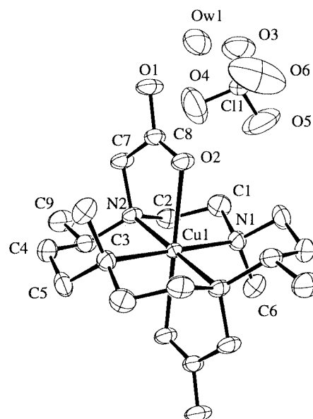
Fig. 5 An ORTEP drawing of the molecular structure of [Cu(H 2 L 9 )][ClO 4 ] 2 ·2H 2 O 7 along with the atom numbering scheme.
